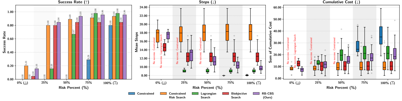
Figure 4: Quantitative performance on the 2D point environment with 10 agents and hard difficulty, plotted as a function of \Delta . Left: Success rate of each method showing that RB-CBS, Constrained Risk Search and Bi-Objective Search sustain high success at most \Delta 's. Center: Average steps to reach goals, where RB-CBS smoothly trades off path length as \Delta increases. Right: Total cumulative cost illustrating that RB-CBS respects tight budgets.
