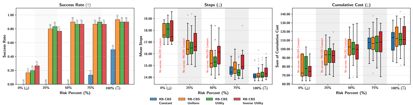
Figure 7: Ablation Study on Initial Risk Allocation Strategies. Comparison of Constant , Uniform , Utility -based, and Inverse Utility -based risk allocation for RB-CBS across four distinct environments (10 Agents, Hard Difficulty). The results consistently demonstrate that dynamic allocation strategies (Uniform, Utility and Inverse Utility) far outperform the rigid Constant approach, especially at tight risk budgets ( \Delta = \underline{\Delta} ). Higher success rates, lower steps and lower costs are better.
