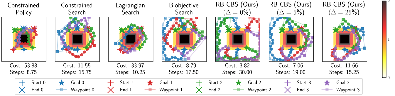
Figure 2: Comparison of different approaches on the 2D navigation problem for a multi-agent setup. Total cumulative cost and average steps count are annotated below each method. Unlike the baselines which cut through high-cost regions leading to riskier paths, our RB-CBS planner coordinates all agents and flexibly adjusts each route to the user-specified \Delta
