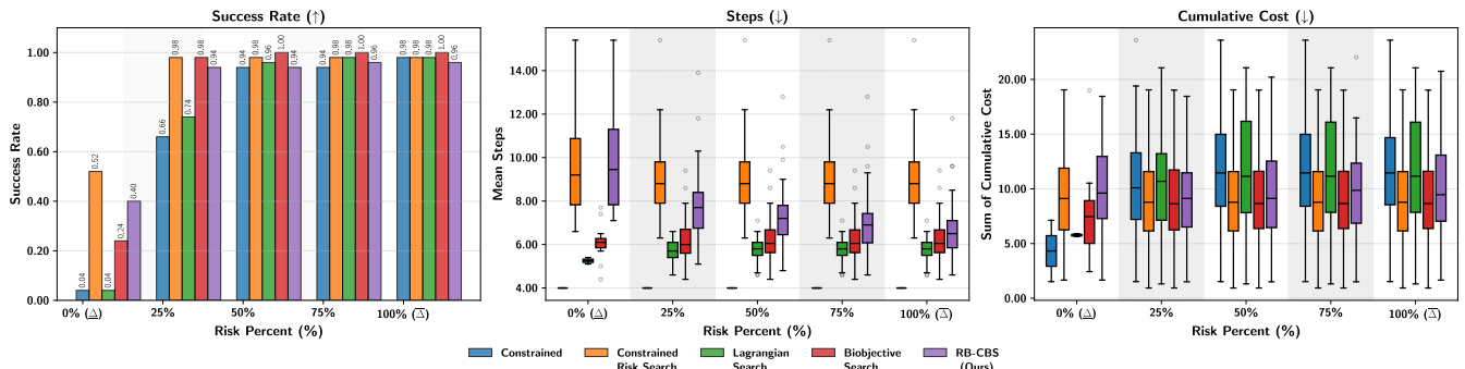
Figure 8: Quantitative results for the 2D Point environment comparing all methods across Easy and Medium difficulties for 5 and 10 agents. These plots visually demonstrate the trade-offs between success rate, steps, and cumulative cost as the risk budget ( \Delta ) is varied. Our method, RB-CBS (purple), consistently shows a strong adaptive profile.
