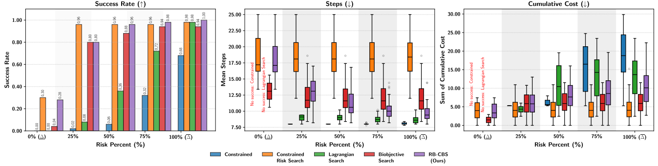
Figure 9: Quantitative results for the 2D Point environment comparing all methods across Hard difficulty for 5 agents. These plots again visually demonstrate the trade-offs between success rate, steps, and cumulative cost as the risk budget ( \Delta ) is varied. Our method, RB-CBS (purple), consistently shows a strong adaptive profile.
