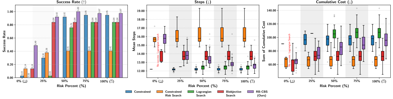
Figure 5: Quantitative results on the visual environment (Scene: SC2 Staging 08) with 10 agents and hard difficulty, as a function of \Delta . Left: Success rate. Center: Average steps showing RB-CBS’s path length decrease as \Delta grows. Right: Total cumulative cost illustrating that RB-CBS respects strict \Delta values. Overall, RB-CBS sustains high success and smoothly trades off cost vs. efficiency across all budgets. See Appendix A.2 for more results on different agent counts, environments and difficulties.
