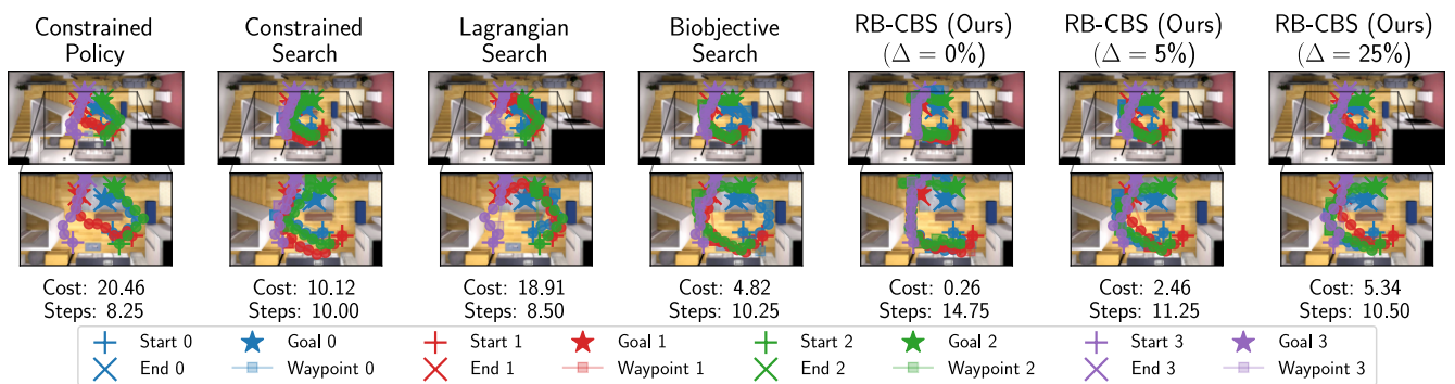
Figure 16: Comparison of different approaches on the visual navigation task for a multi-agent setup. Total cumulative cost and average steps count are annotated below each method. Our RB-CBS planner flexibly trades off efficiency and safety via the user-specified \Delta while coordinating multiple agents to reach their goals.
