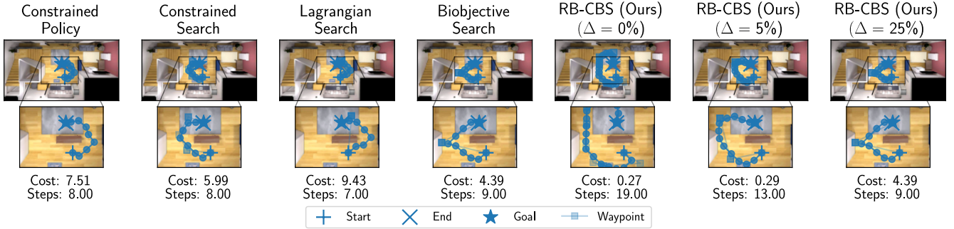
Figure 3: Single-agent trajectory comparison on the visual navigation task. Total cumulative cost and average steps count are annotated below each method. Our RB-CBS planner flexibly trades off efficiency and safety via the user-specified \Delta . (See Appendix 16 for the corresponding multi-agent trajectory comparison.)
