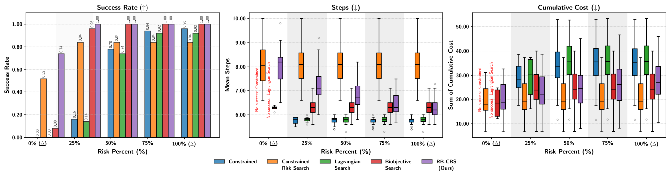
Figure 11: Quantitative results for the visual navigation environment on SC2 Staging 08 scene comparing all methods across Easy and Medium difficulties for 10 agents.
