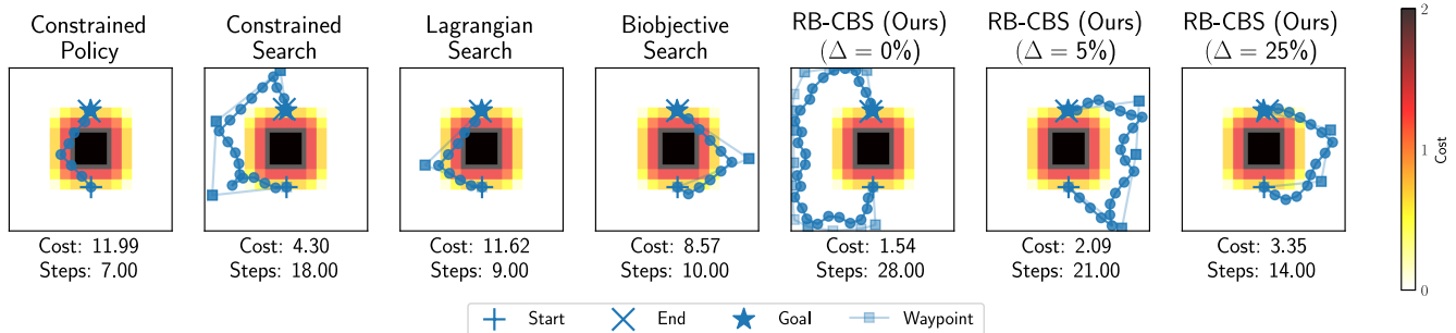
Figure 1: Comparison of different approaches on the 2D navigation problem for a single agent setup. Total cumulative cost and average steps count are annotated below each method. While standard baselines often cut directly through high-cost regions leading to riskier paths, our RB-CBS planner flexibly trades off efficiency for safety by adapting its route to user-specified \Delta .
